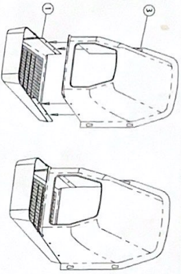
Figure 1: Align holes of the basket and nesting box as shown.
